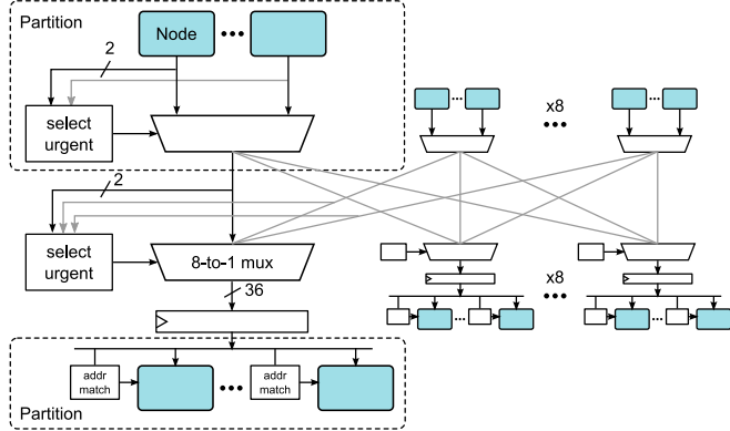
Figure 4: DART's global interconnect. Nodes are grouped into partitions so the crossbar needed is small
